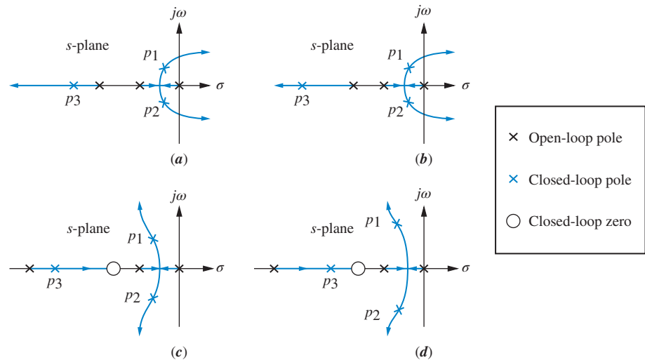
FIGURE 8.20 Making second-order approximations
