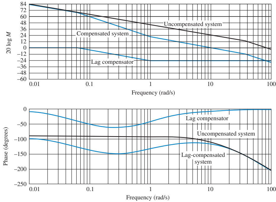
FIGURE 11.6 Bode plots for Example 11.2
