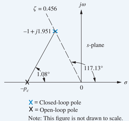
FIGURE 9.67 Locating compensator pole
