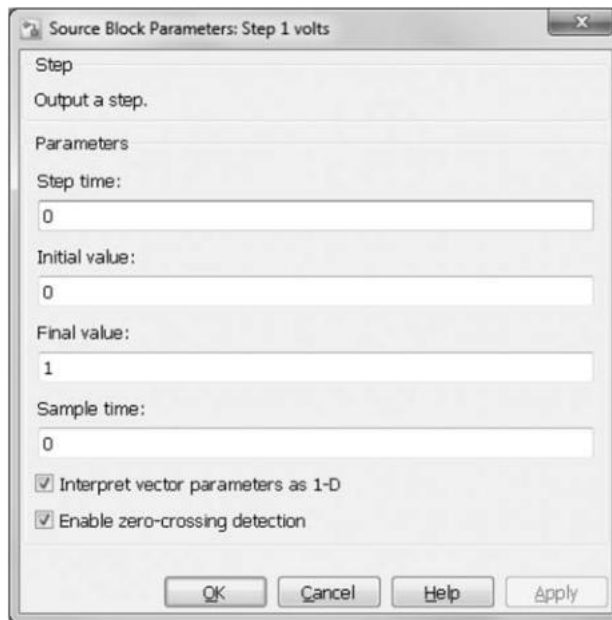
FIGURE C.6 Block parameters windows for a. 1-Volt step source; (figure continues)
