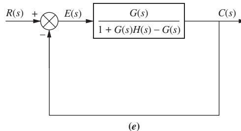
FIGURE 7.15 Forming an equivalent unity feedback system from a general nonunity feedback system
