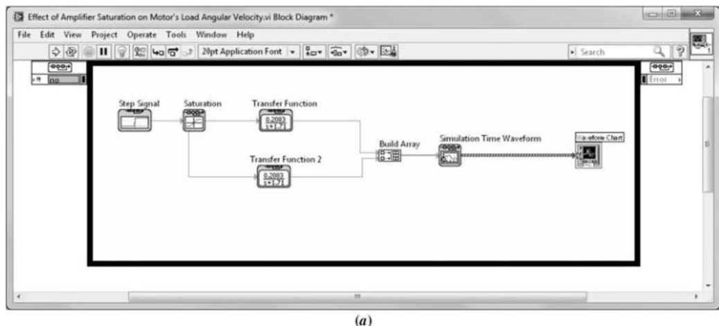
FIGURE D.20 Simulation of a dc motor with and without saturation: a. Block Diagram ; (figure continues)
