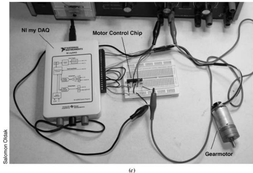
FIGURE D.26 (Continued) b. basic configuration showing NI myDAQ interfaced with motor control chip and gearmotor; c. interconnected hardware
