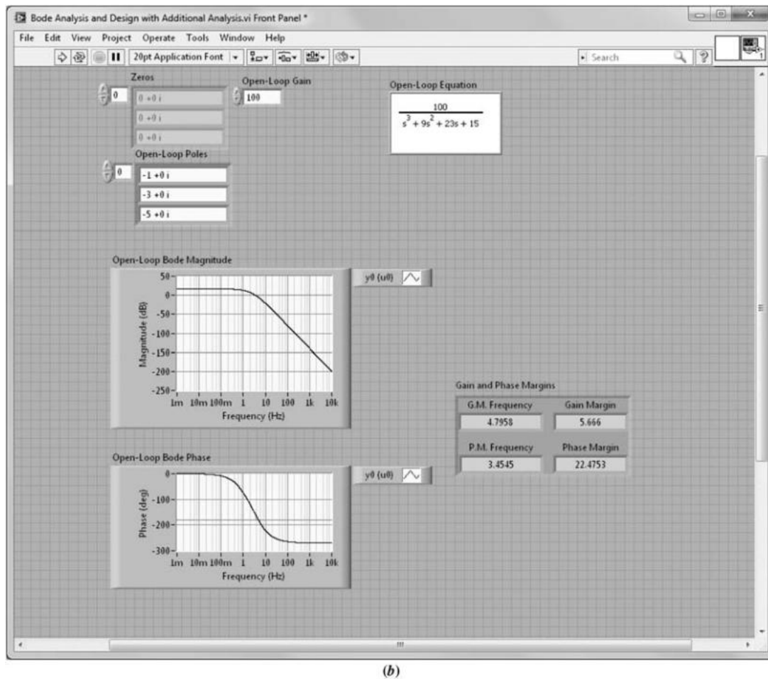
FIGURE D.17 (Continued) b. Front Panel
