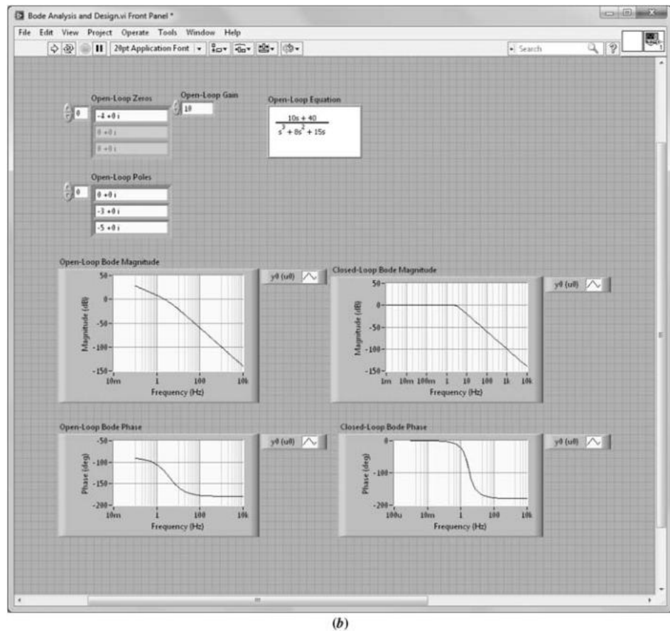
FIGURE D.16 (Continued) b. Front Panel
