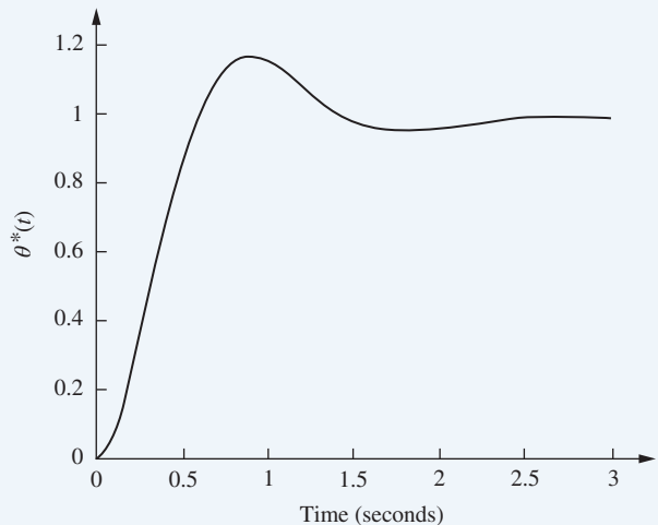
FIGURE 13.35 Closed-loop digital step response for antenna control system with a lead compensator
