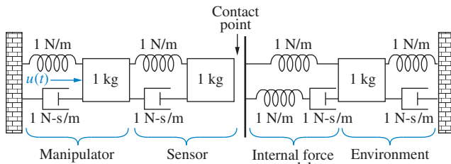
FIGURE P3.14 Robotic manipulator and target environment 11
