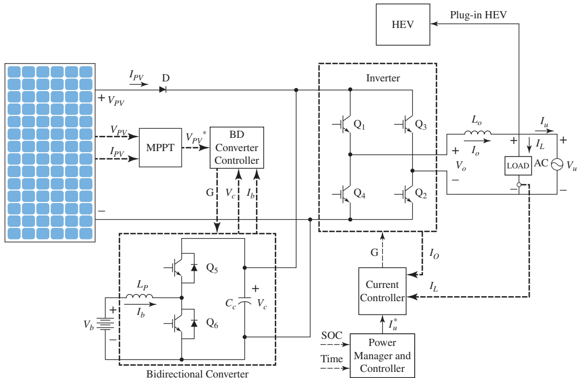
FIGURE P1.5 Proposed solar powered residential home with plug-in hybrid electric vehicle (PHEV) loads 8
