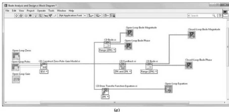
FIGURE D.16 Bode analysis via LabVIEW: a. Block Diagram ; (figure continues)
