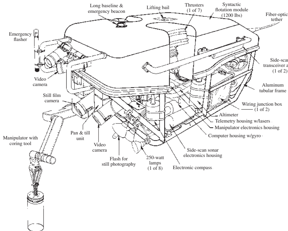
FIGURE 6.9 Jason is an underwater, remote-controlled vehicle that has been used to explore the wreckage of the Lusitania . The manipulator and cameras comprise some of the vehicle's control systems (Courtesy of Woods Hole Oceanographic Institution)
