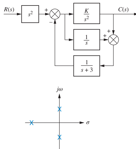
FIGURE P6.10 Closed-loop system with pole plot
