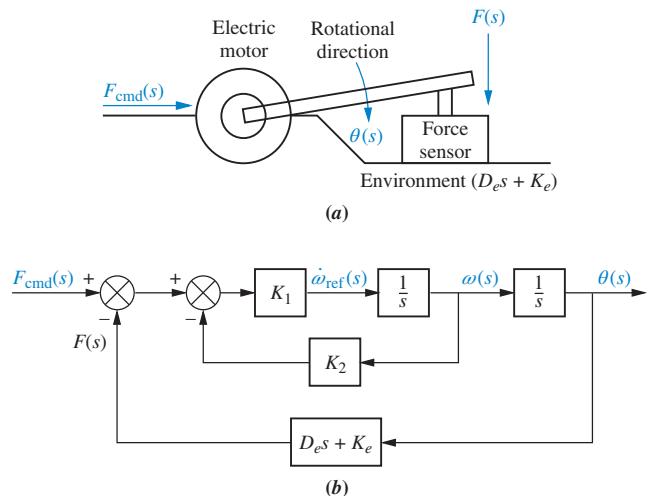
FIGURE P7.30 a. Force control mechanical loop under contact motion; 10 b. block diagram 10
