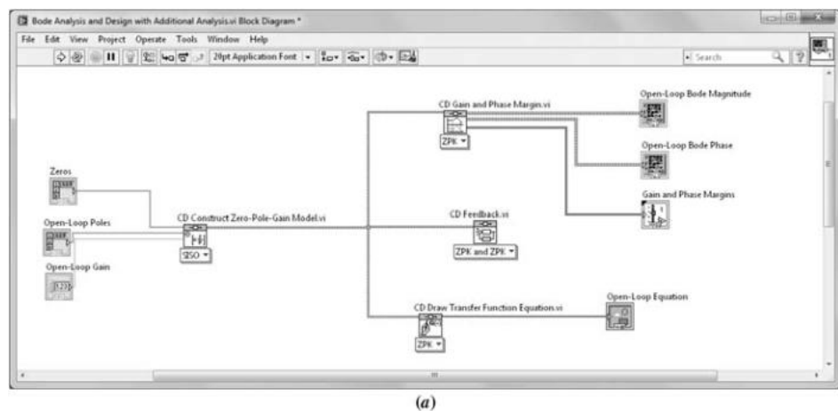
FIGURE D.17 Bode analysis with gain and phase margin: a. Block Diagram; (figure continues)
