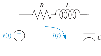
FIGURE P1.7 RLC network
