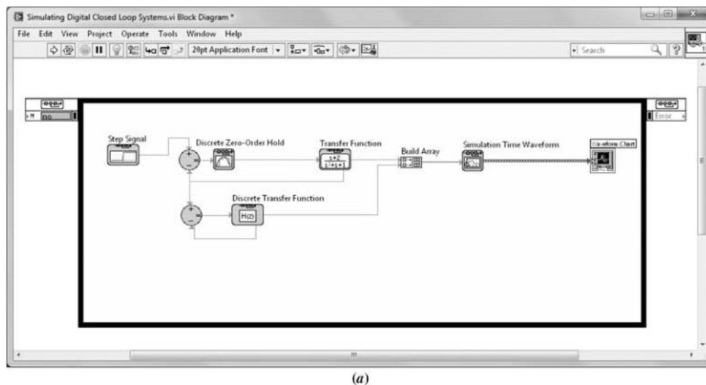
FIGURE D.23 Simulation of digital systems with Simulation palette: a. Block Diagram ; (figure continues)
