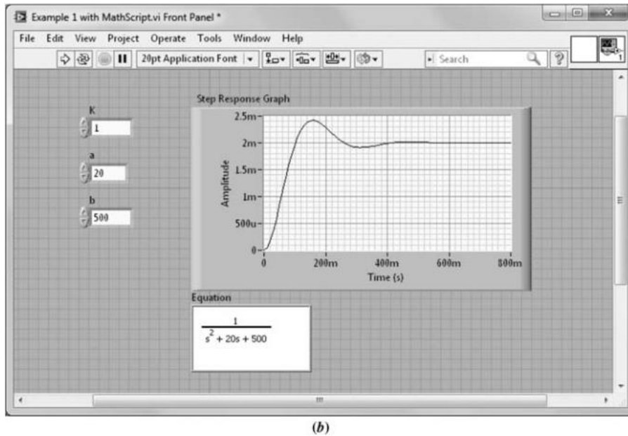
FIGURE D.9 (Continued) b. for block diagram in Figure D.7(b)
