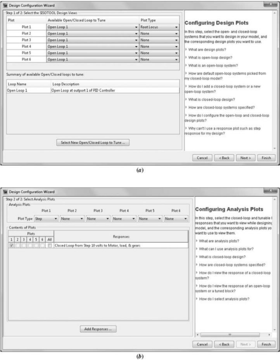
FIGURE C.24 Design Configuration Wizard: a. with root locus selected as the design tool; b. with closed-loop step response selected as analysis tool
