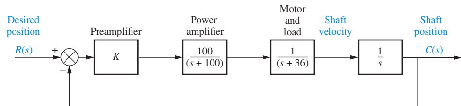
FIGURE 11.2 System for Example 11.1
