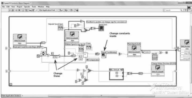
FIGURE P9.15 (Continued) b. Block Diagram
