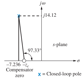
FIGURE 9.52 Finding the compensator zero in Example 9.7
