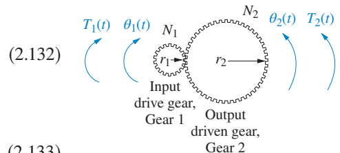
FIGURE 2.27 A gear system
