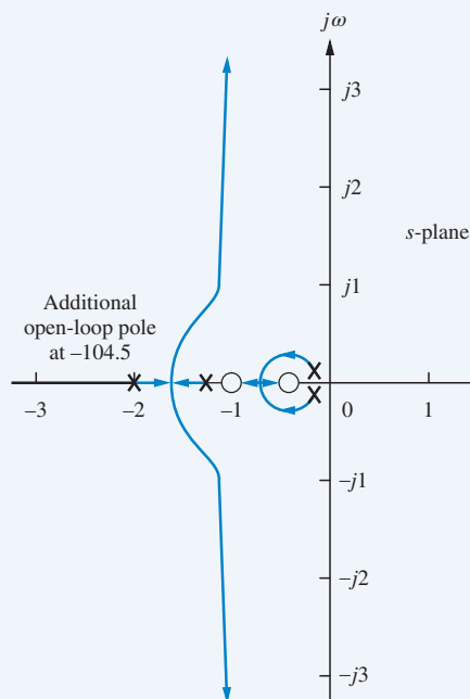
FIGURE 9.68 Root locus for lead-compensated system
