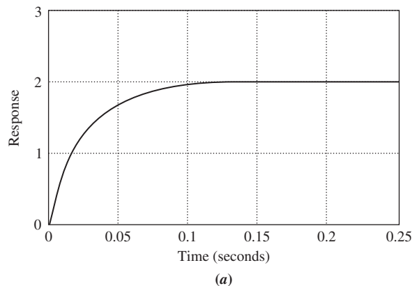
FIGURE P4.10 (figure continues)
