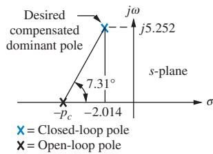
FIGURE 9.27 s -plane picture used to calculate the location of the compensator pole for Example 9.4
