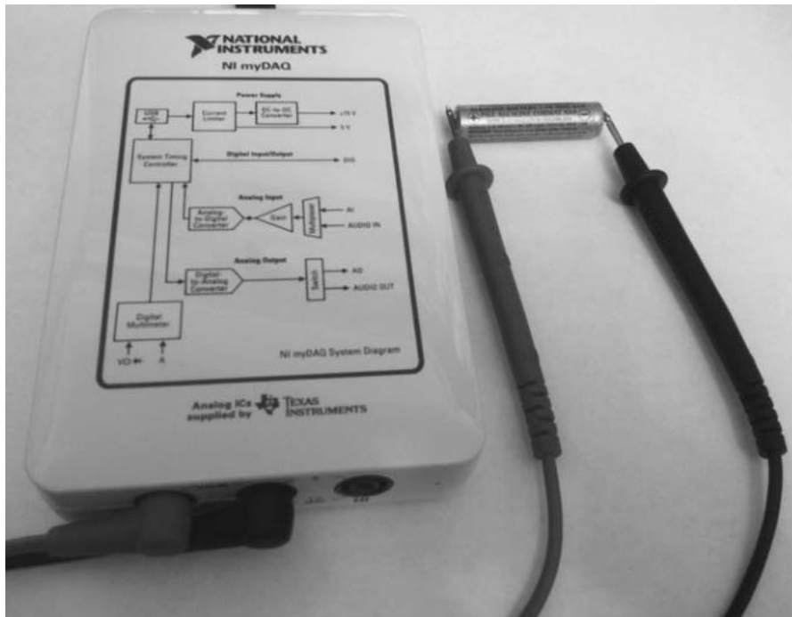
FIGURE D.28 Battery voltage measurement: a. Connections to myDAQ; (figure continues)
